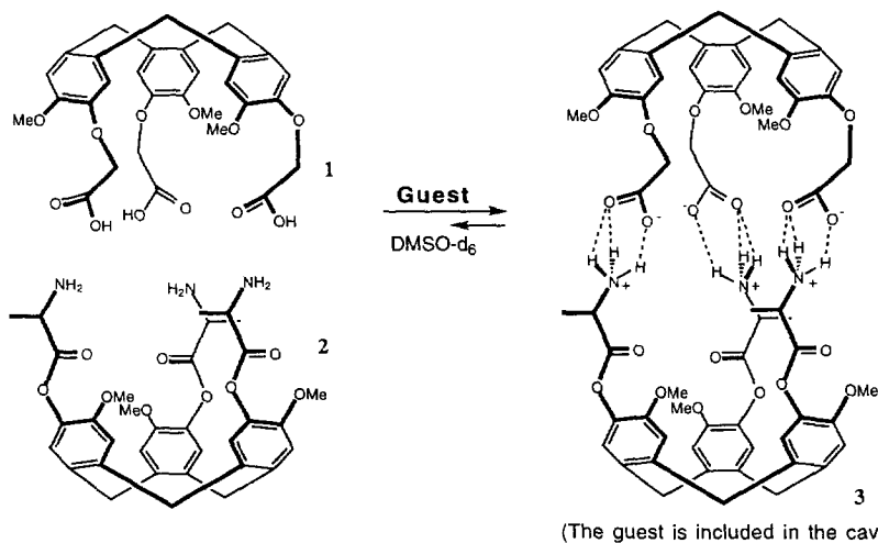
Figure 1. Self-Assembly based on the charged hydrogen bonding interaction between CTV trisidic ( 1 ) and CTV trisamine ( 2 ).
